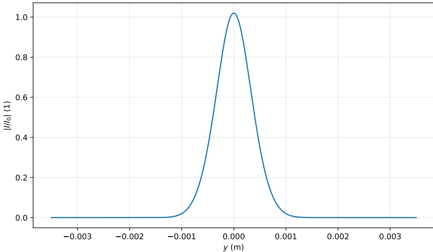
Intensity profile I(x=0, y, z=0.478)/I_0 , P_{in}=0.4P_{cr} , artificial time
